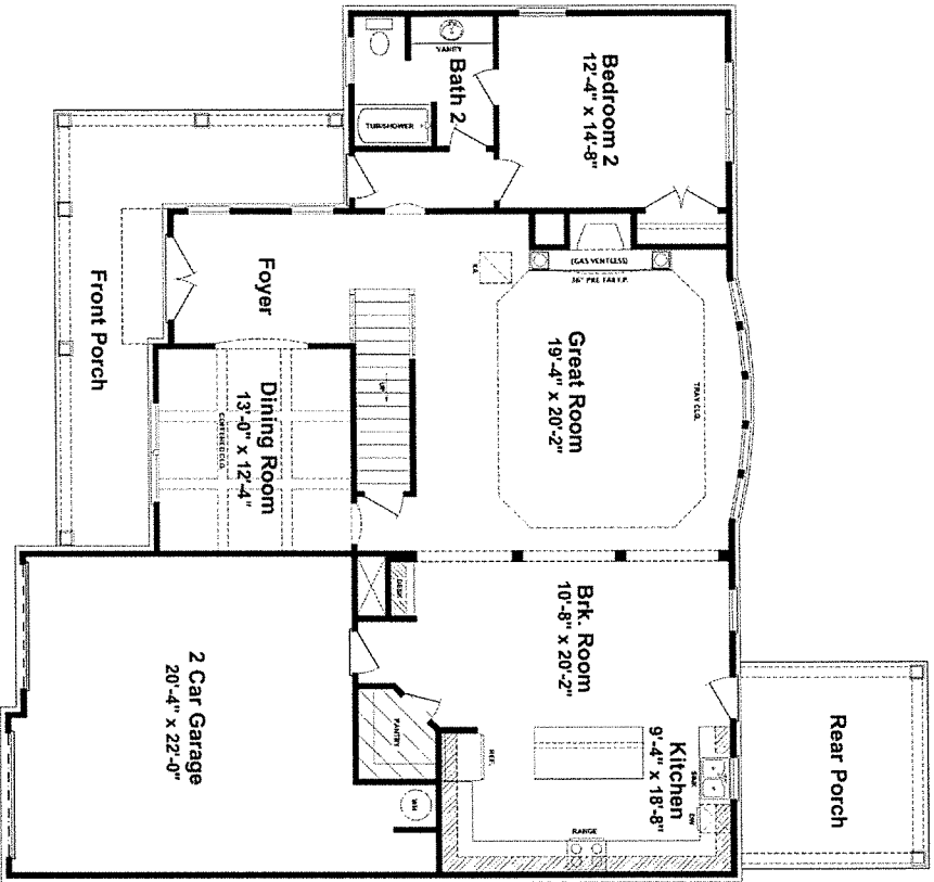
First Floor 56'-4" x 59'-8"
